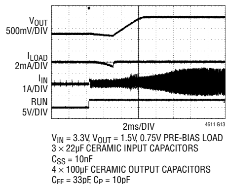
Start-Up, Pre-Bias
